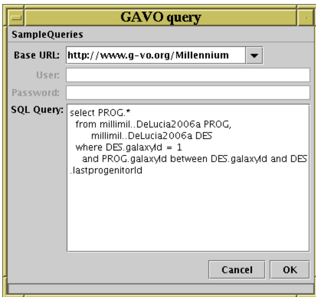
GAVO load dialogue with an example query on the milli-Millennium database
