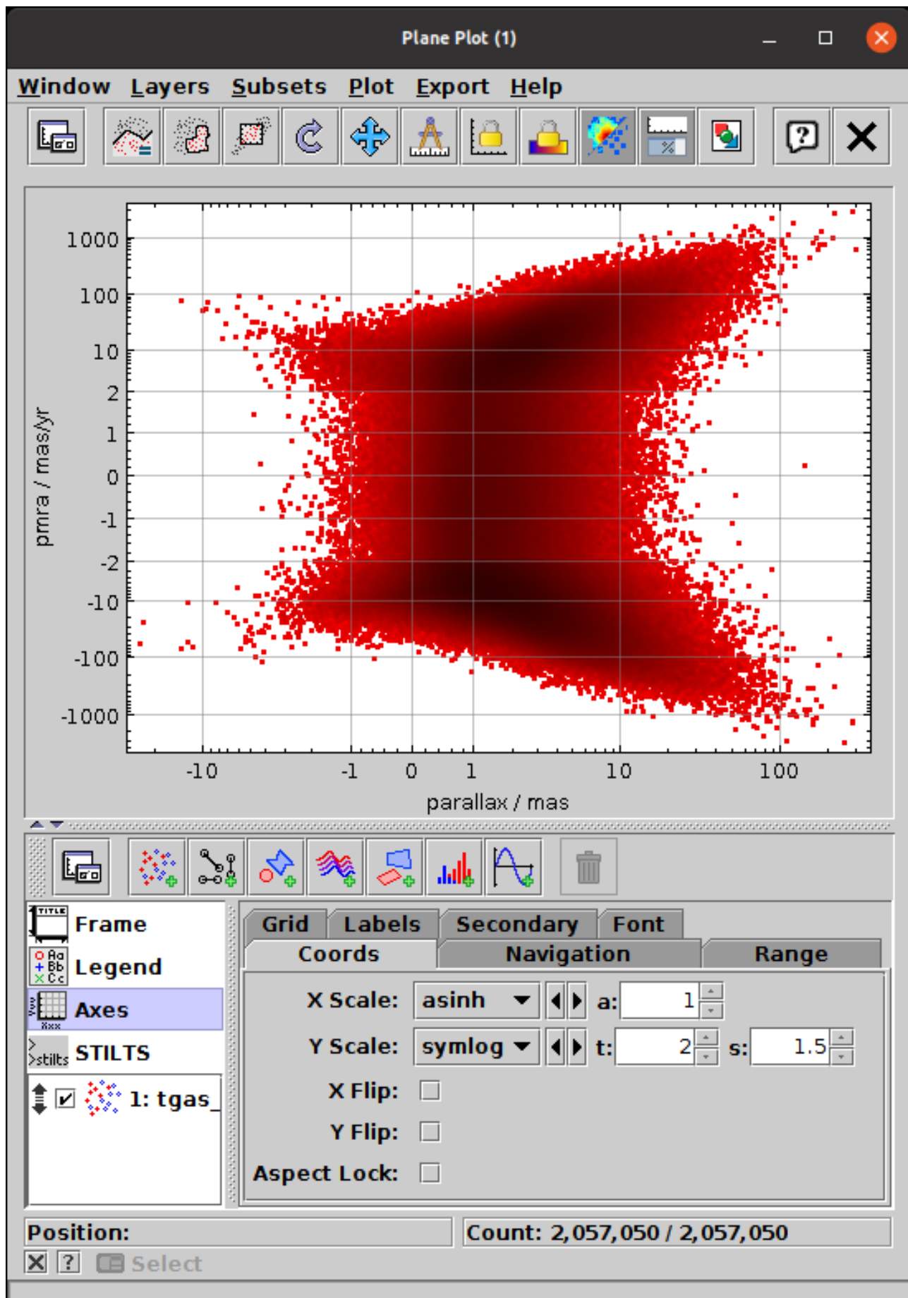
2d scatter plot using asinh and symlog axis scalings
