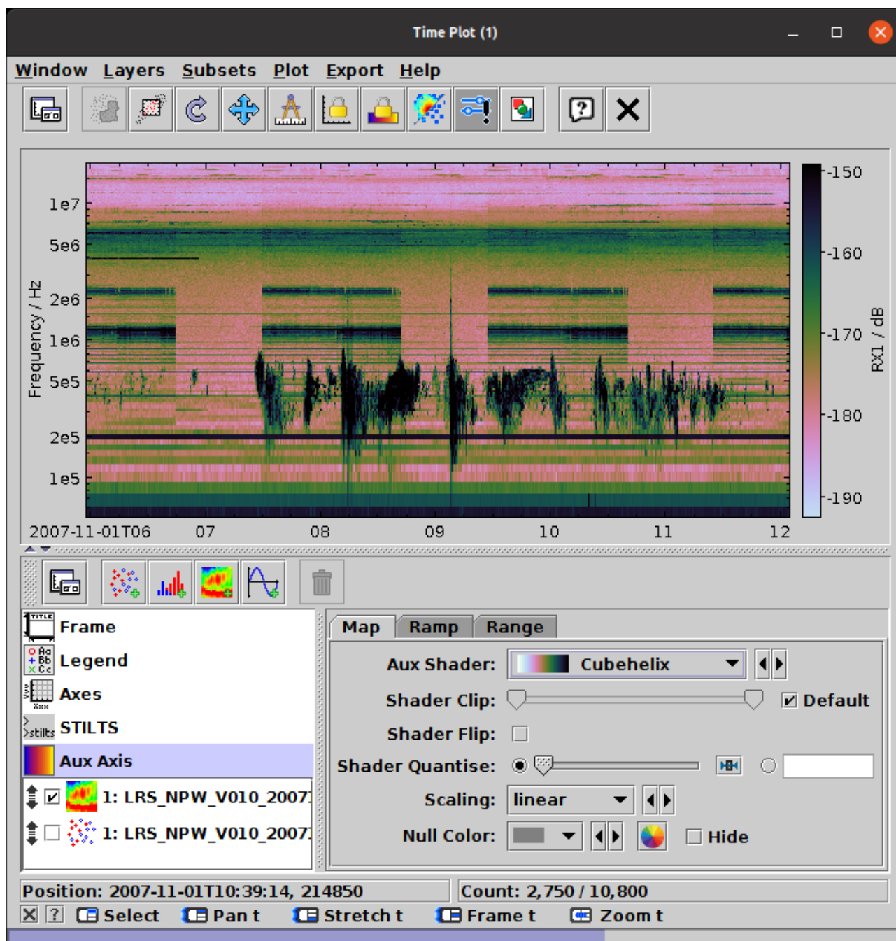
Time Plot window with a Spectrogram layer
