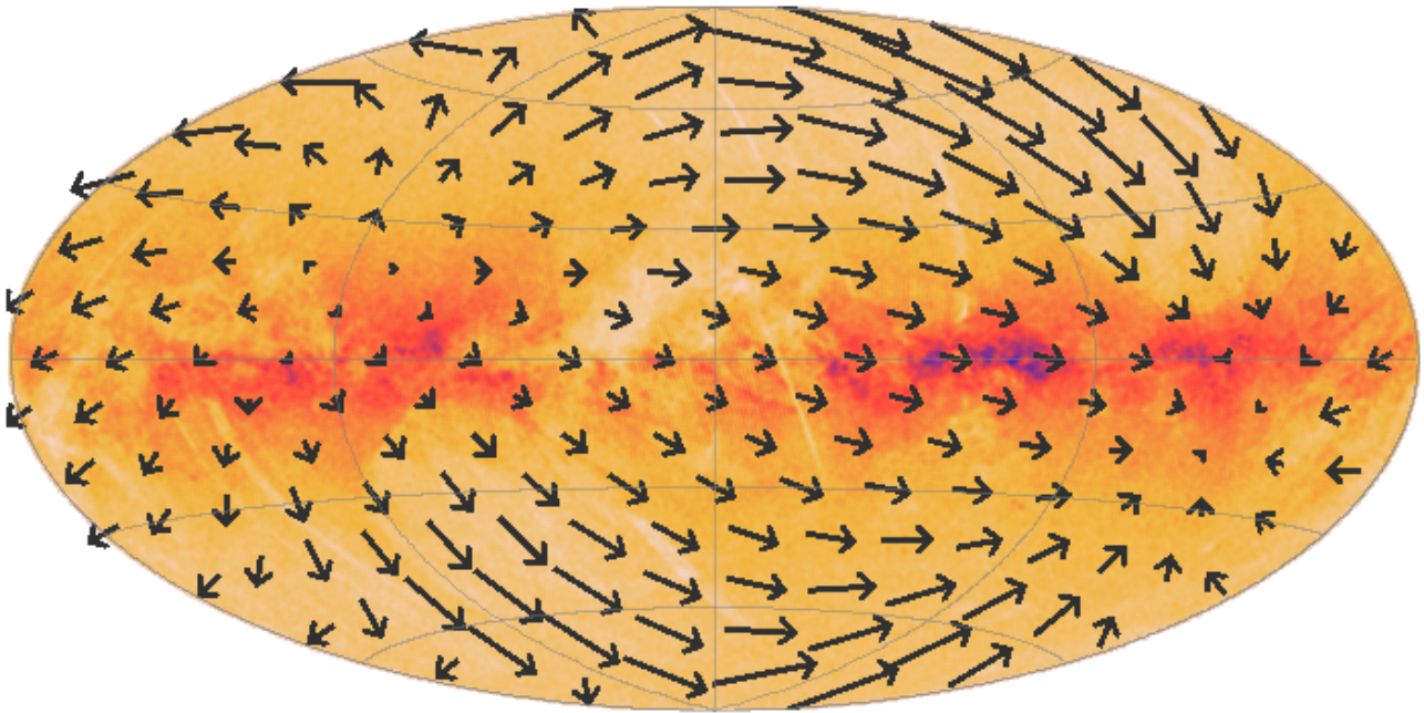
Example SkyVecField plot
