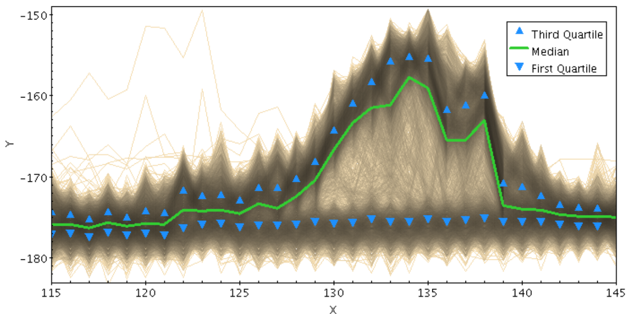
Example StatMark plot
