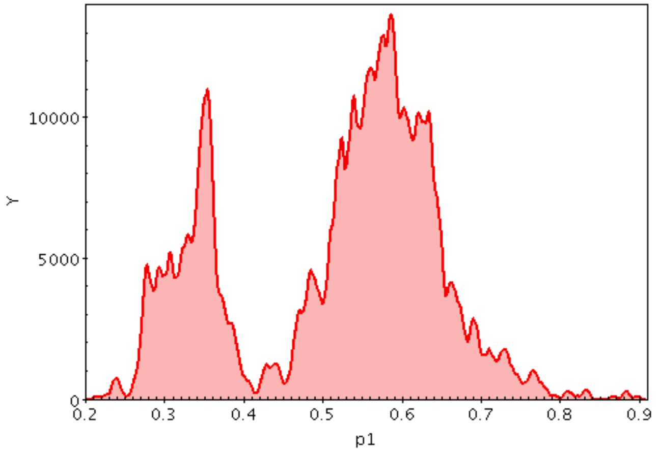
Example KDE plot
